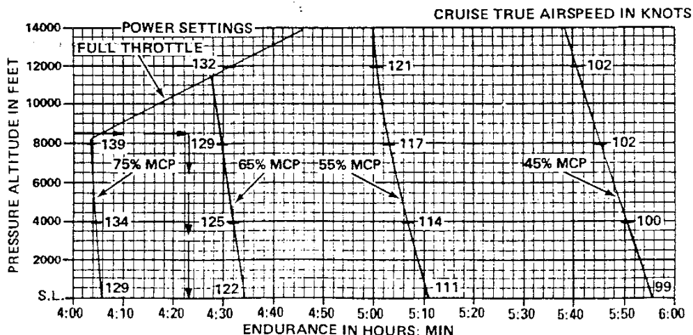
Figure 5-15. Endurance Profile — 51 Gallons Fuel
