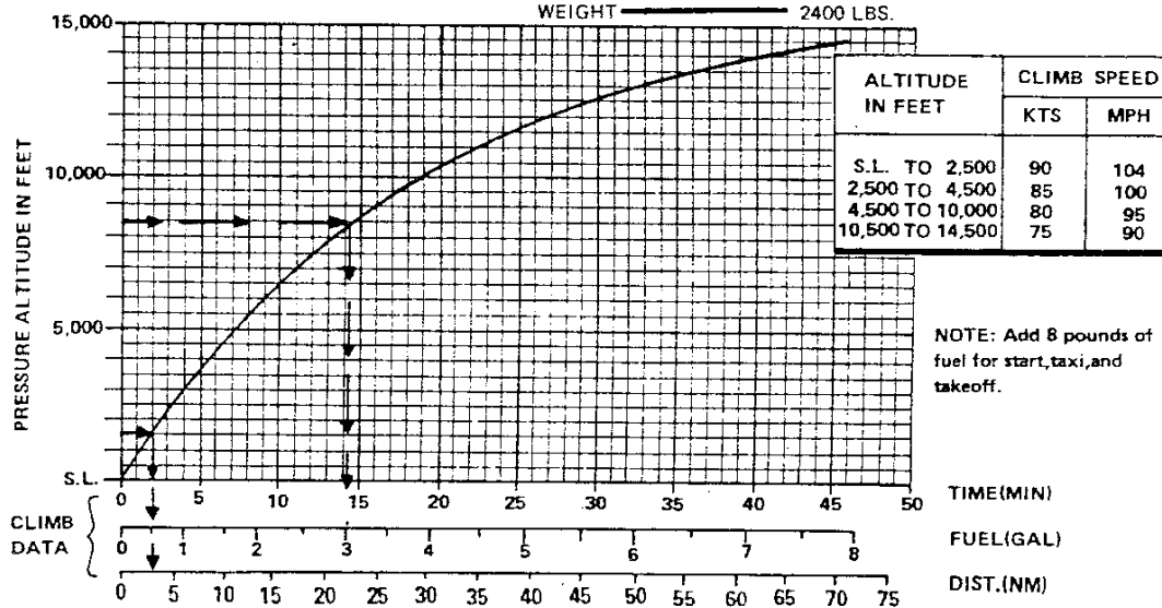
Figure 5-9. Time Fuel and Distance to Climb
