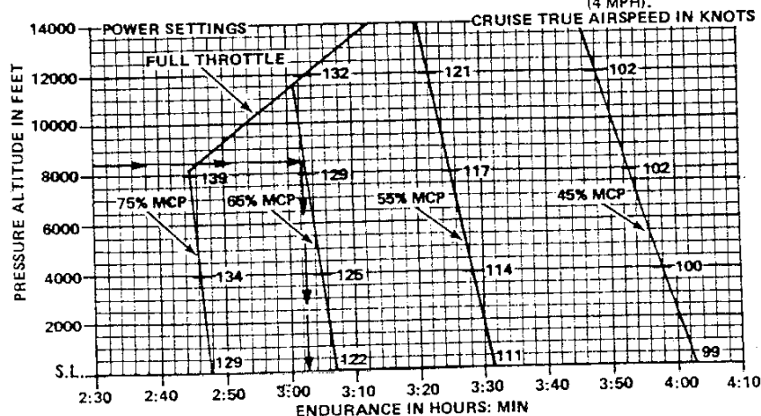
Figure 5-14. Endurance Profile — 37 Gallons Fuel
