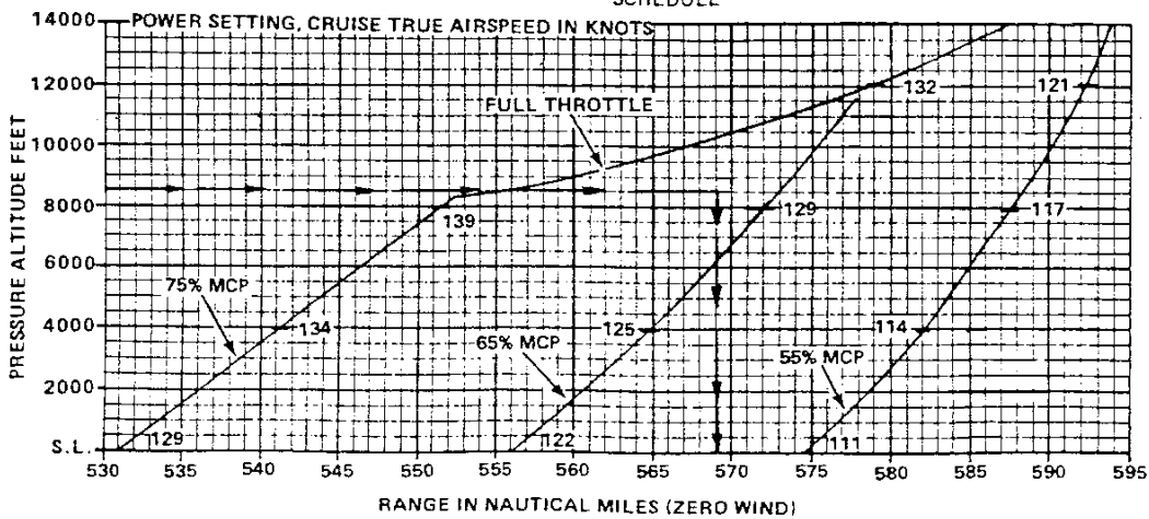
Figure 5-13. Range Profile - 51 Gallons Fuel
