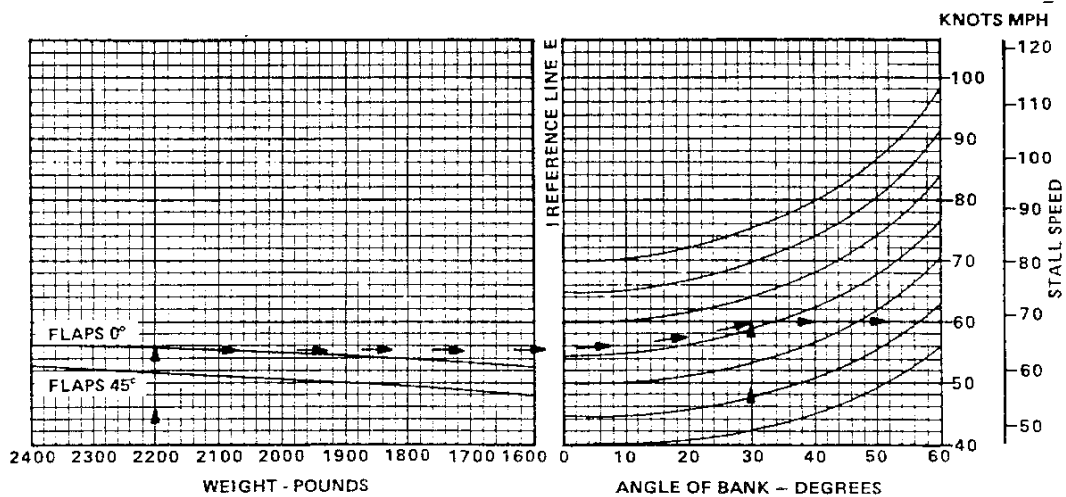
Figure 5-5. Stall Speeds
