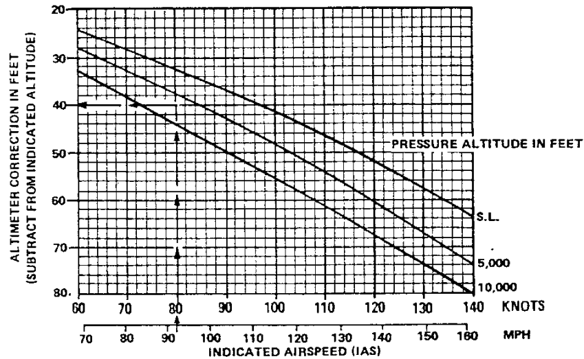
Figure 5-4. Altimeter Correction - Alternate System
