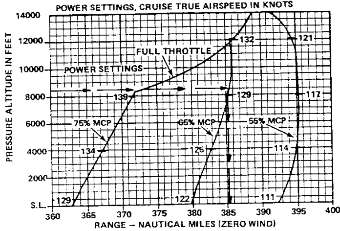
Figure 5-12. Range Profile-37 Gallons Fuel
