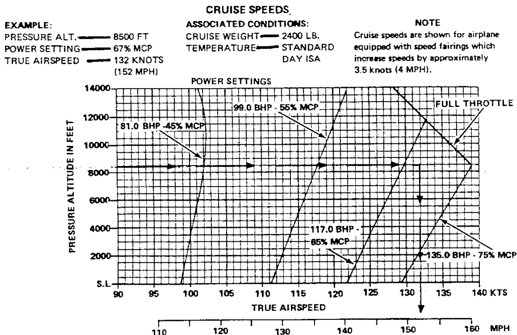
Figure 5-11. Cruise Speeds
