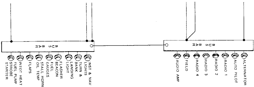
Figure 7-3 Electrical System (Sheet 2 of 2) Revised: December 15, 1977 7-1Ga/(7-16b blank)
