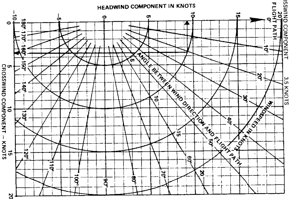
Figure 5-6. Crosswind Component Chart
