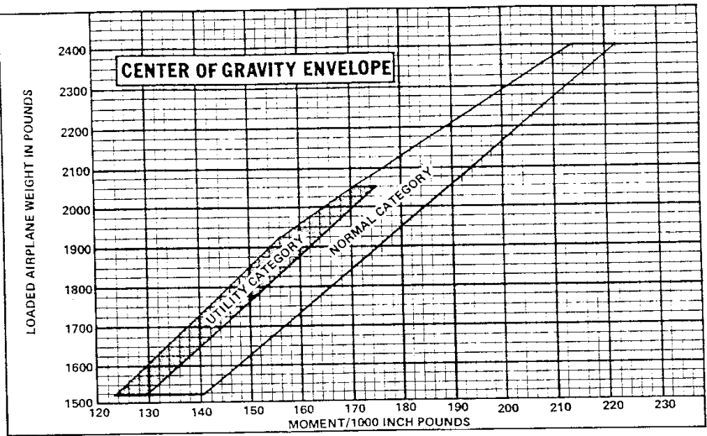
Figure 6-5. Center of Gravity Envelope
